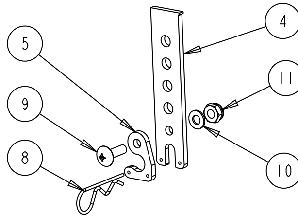
CABLE MNT ASSY (FC-063) SCALE 0.500
